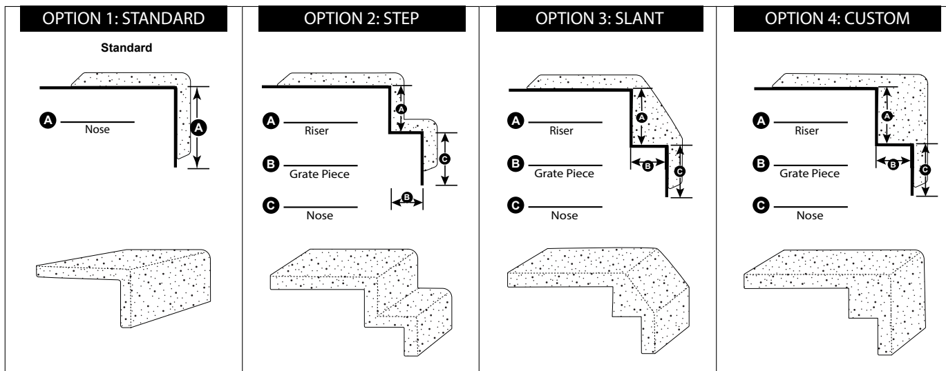
Side Views
